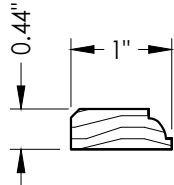
4 GLAZING BEAD
