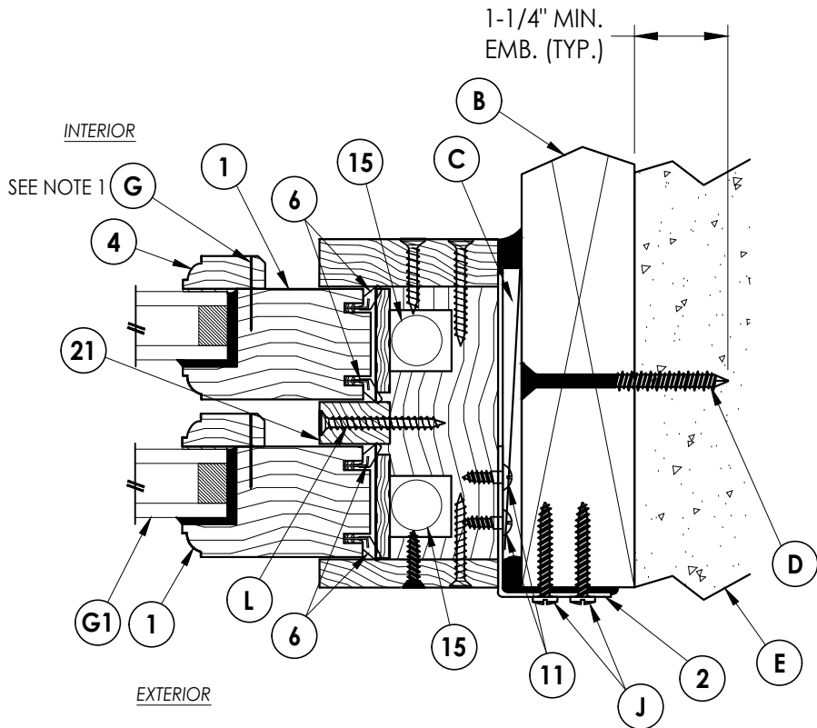
3 HORIZONTAL CROSS SECTION 2 2X Buck Construction (Anchor Clip Installation)
