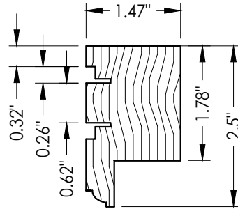
12 TOP RAIL Bottom sash
