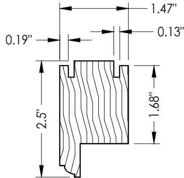
24 TOP RAIL Top sash
