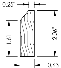
14 SILL EXTENDER
